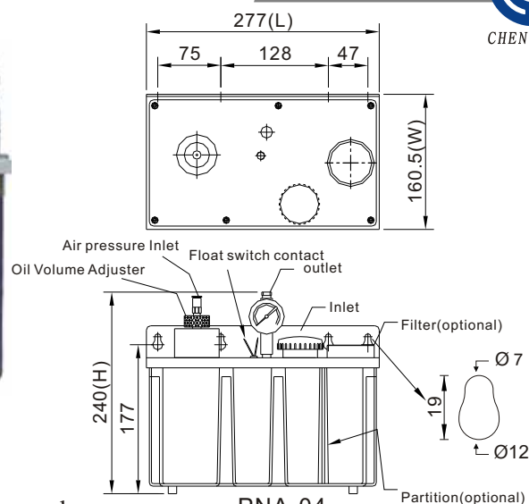
PNA-04 Type Standards Externals
