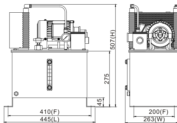
CLST-20 Type Standards Externals
