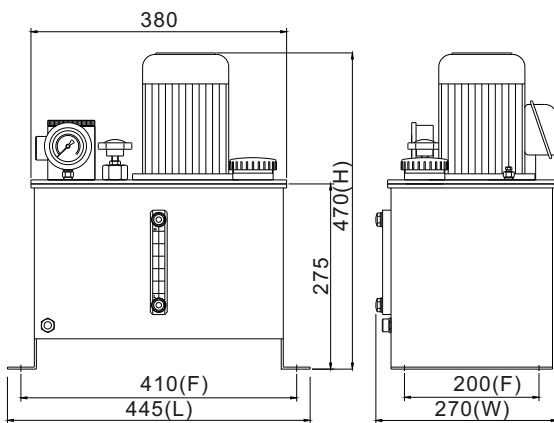
CLSA-20 Type Standards Externals
