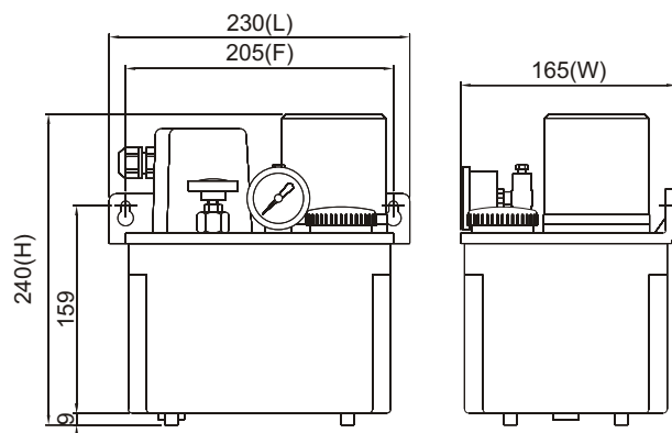
CEVB-03 Type Standards External
