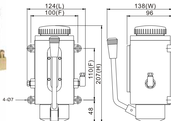
CLA-8 Type Standards External
