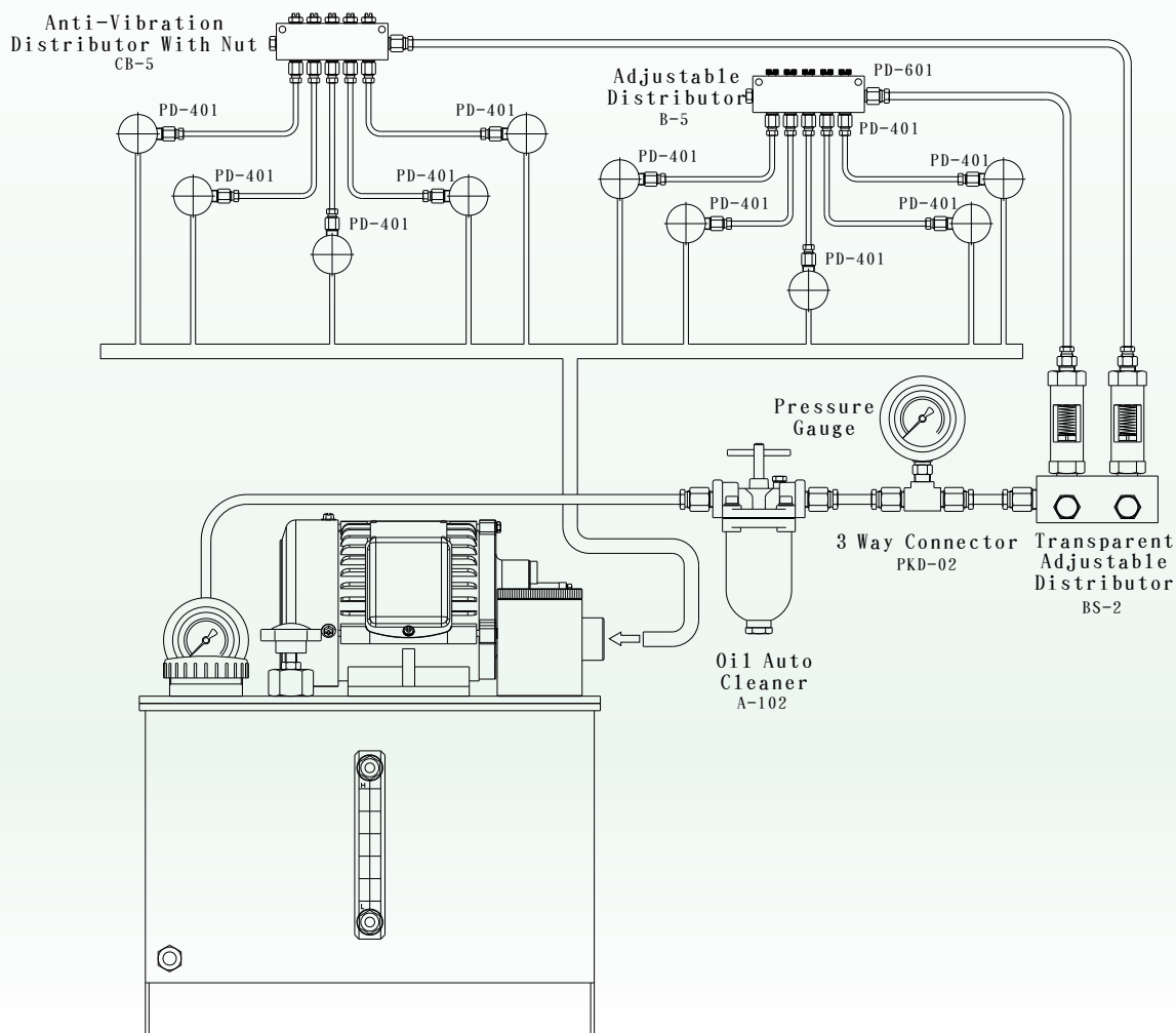
The Piping of CLSB-20L Type Circulating Lubrication System
