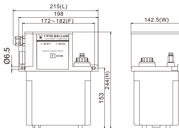
CESD-01 Type Standards External
