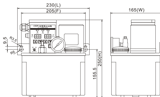
COA-03 (25W) Type Standards External
