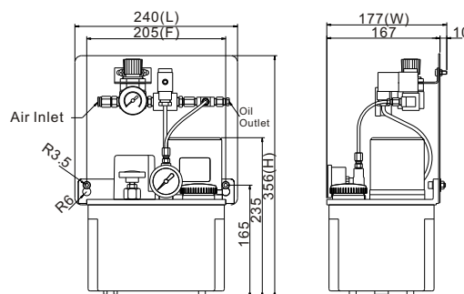
CEN25-03 Type Standards Externals
