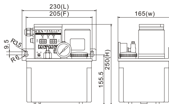
CENA-03 Type Standards Externals
