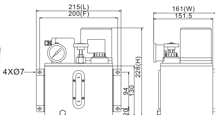
CEV-02(25W) Type Standards Externals
