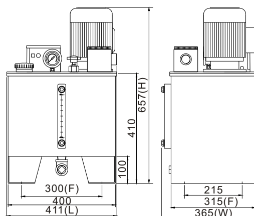
CLS 10-30 Type Standards Externals
