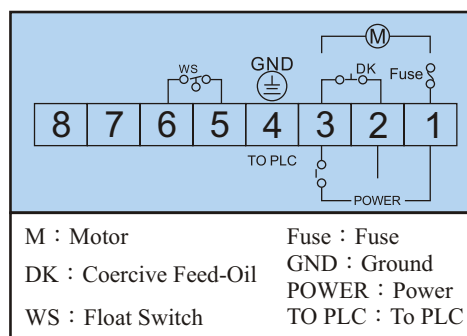
CESG-03Type Single Phase Wiring Diagram
