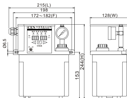
CEN04-01 Type Standards External
