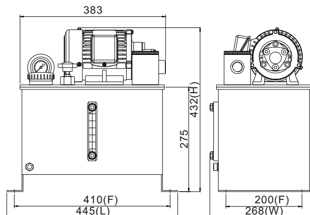
CLSB-20 Type Standards Externals
